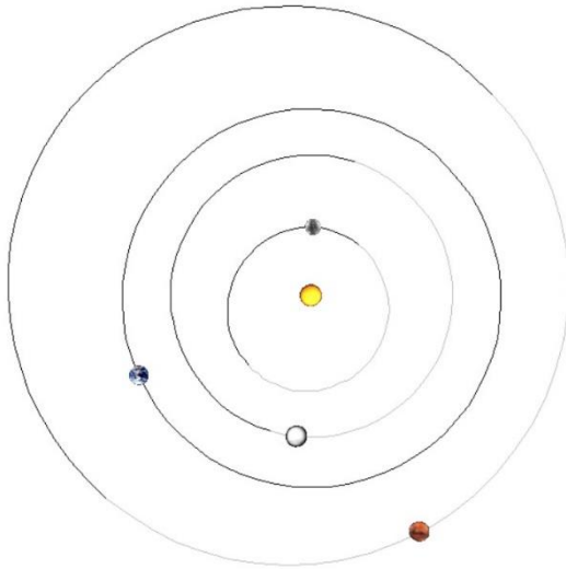
Solar System: Fri 2022 Apr 15 13:00
