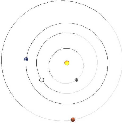
Solar System: Tue 2022 Mar 15 13:00
