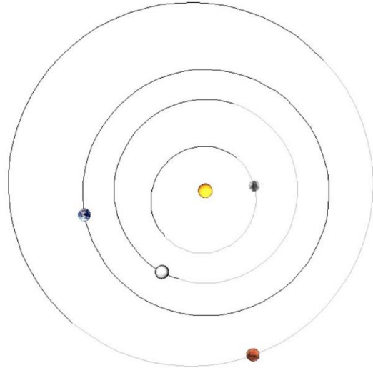
Solar System: Fri 2022 Apr 1 13:00
