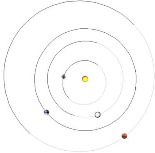
Solar System: Sun 2022 May 1 13:00
