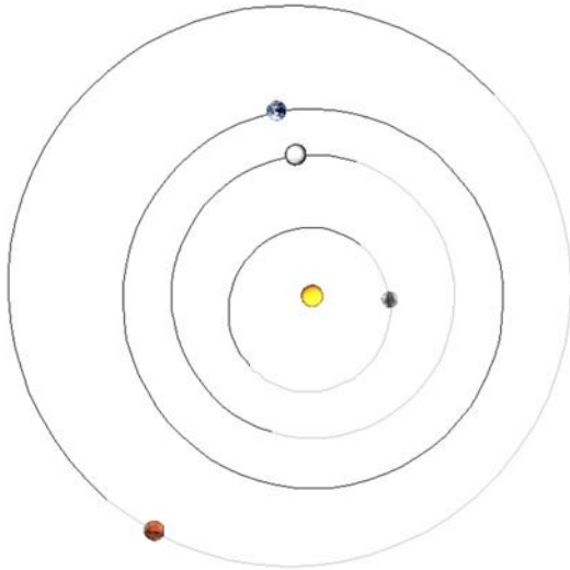
Solar System: Sat 2022 Jan 1 13:00
